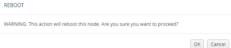
Figure 25 Reboot Dialog
